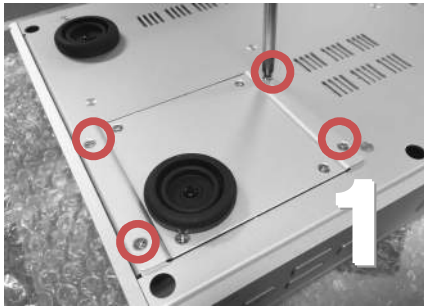
Carefully remove the outer four Phillips screws
