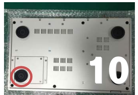
Screw the battery holder plate (outer four) screws in place, making sure the foot is positioned in the lower, outside corner.
